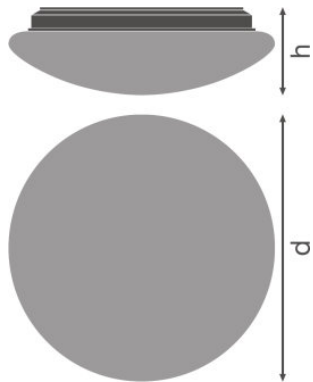
SF CIRCULAR 250 S 13 W 3000 K IP44 WT, SF CIRCULAR 250 S 13 W 4000 K IP44 WT
